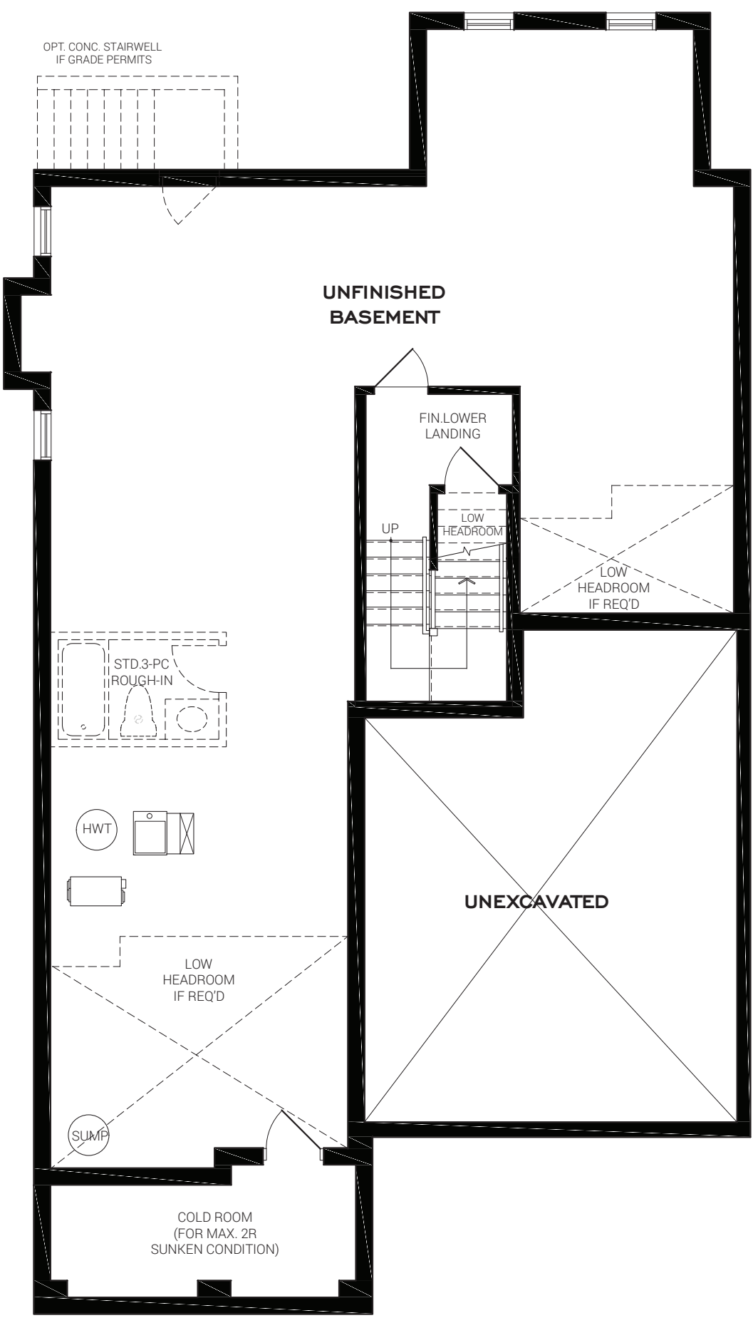
BASEMENT LEVEL ELEV. A
